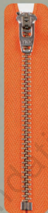
YMRNC-39 GSN8(C5) 三号Y型亮银半自动头(C5)闭口拉链 抗镍 No.3 Metal Y-type shiny silver-metal Anti-nickel closed-end with "C5" finish Semi-auto-lock slider
