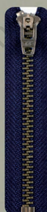
YGTHC-49 GSN8(H3) 四号Y型古银半自动头(H3)闭口拉链 No.4 Metal Y-type antique silver closed-end with "H3" finish Semi-auto-lock slider
