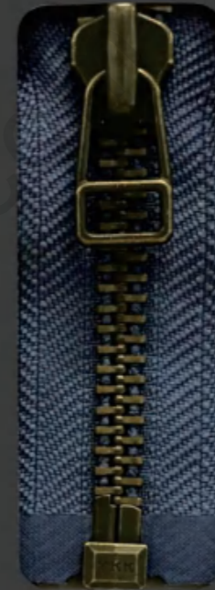
MGMKBOR-86 DADHR (I) 八号金属青古铜牙开尾拉链 DADHR 自动头 NO.8 Metal antique brass open-end with "I" finish auto-lock slider
